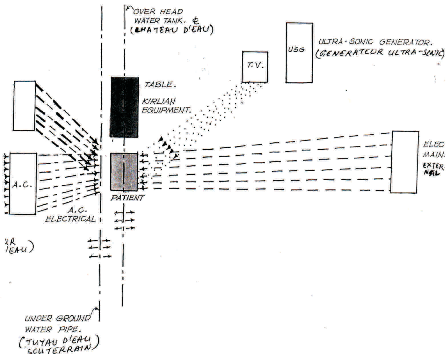
ROOM LAY OUT.
